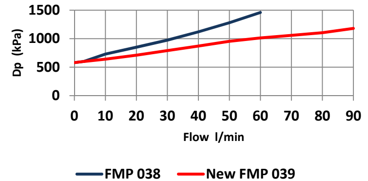
\Delta p By-pass FMP 38 Vs. New FMP 039 Oil viscosity 30 cst.
