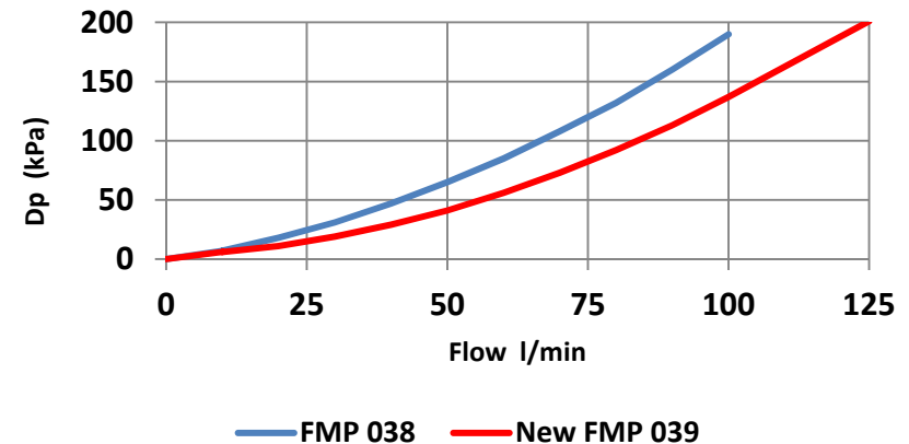
\Delta p Body FMP038 Vs. new FMP 039 oil density 0.86
